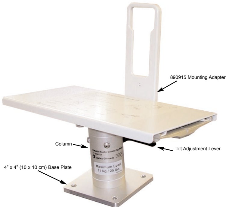
Light monitor mounted on a counter top mount, P/N: 8000726. Requires Datex-Ohmeda supplied mounting adapter, P/N: 890915.
